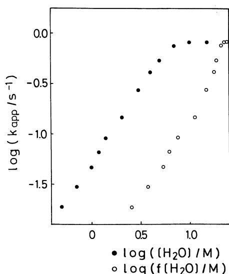
Fig. 12. Activity correction for \log(k_{app}/s^{-1}) vs. \log([H_2O]/M) plot in the reaction of DPA^{+\cdot} with water.
